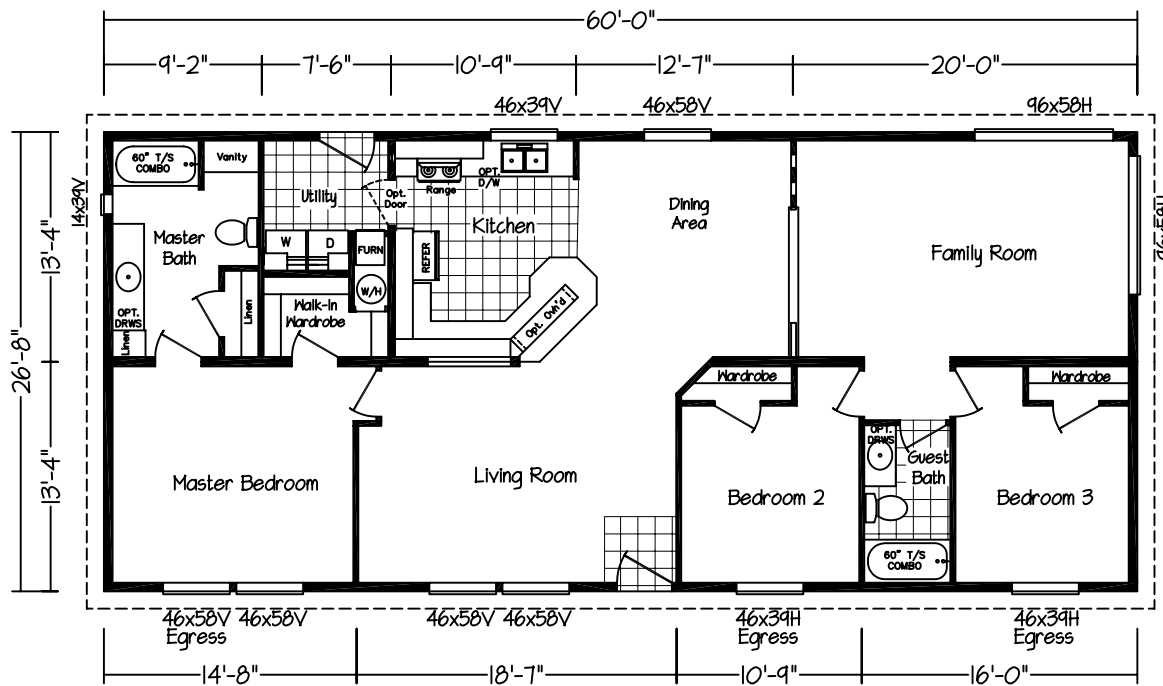
Model: KBSE-60173 1600 Sq. Ft. 3 Bedroom 2 Bath
